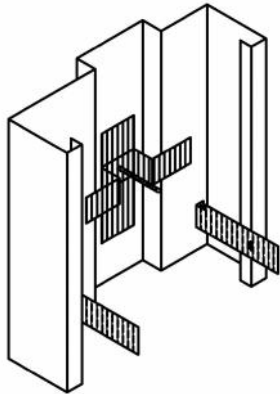
Compression Anchor (CO) Standard
