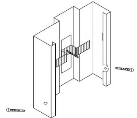
Compression Anchor (CP) Optional
