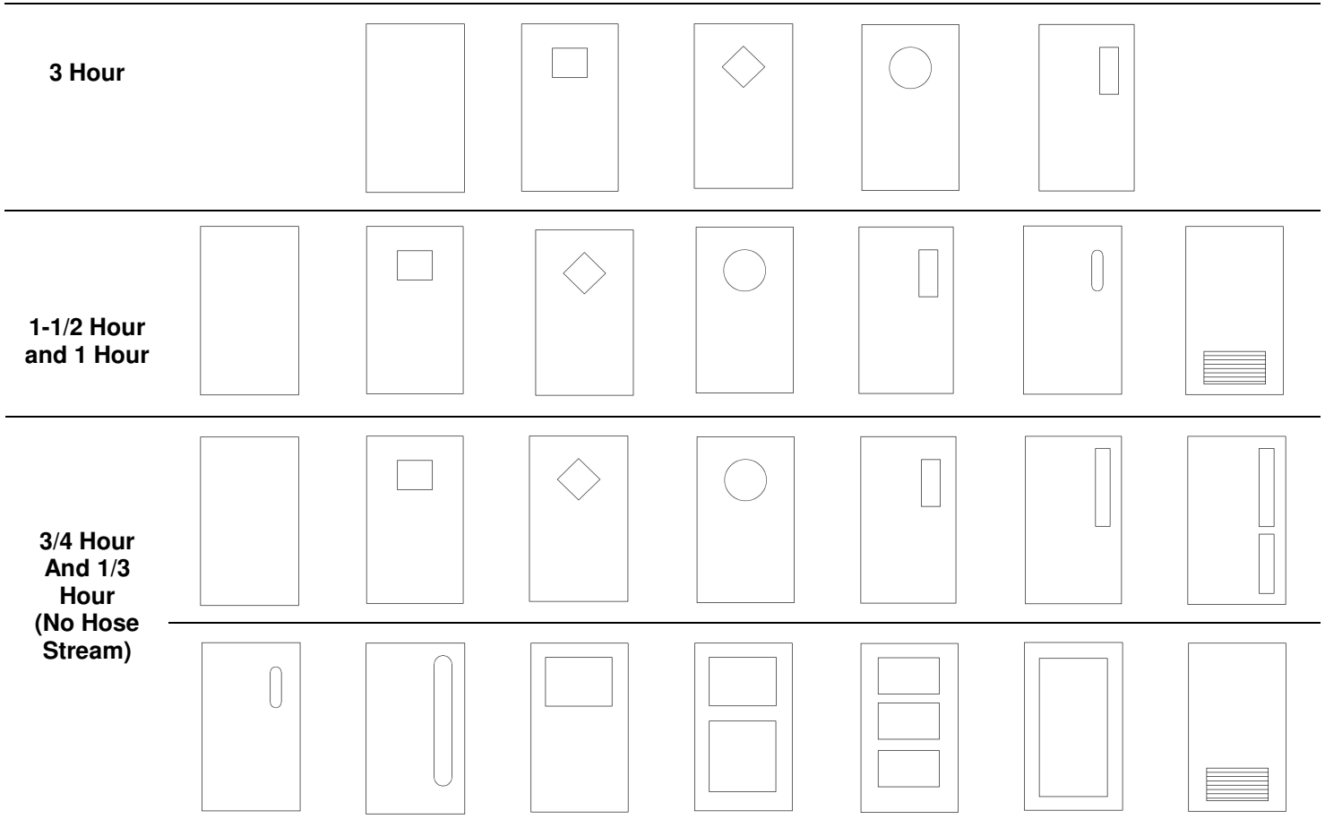
Labeled Glazing Materials for Hollow Metal Fire Doors (from NAAMM/HMMA)
