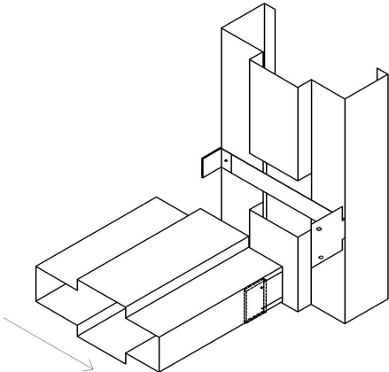
Side or Top Mounting Bracket
