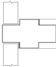
Welded or Removable Mullion Between Doors
