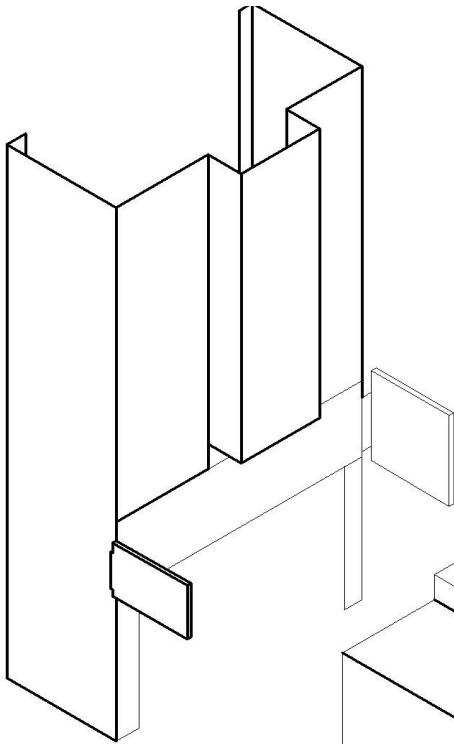
Splice Joint for Jamb to Mullion
