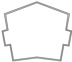
Angled Mullion 1
