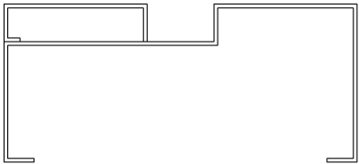
Center Glazed Single Rabbet
